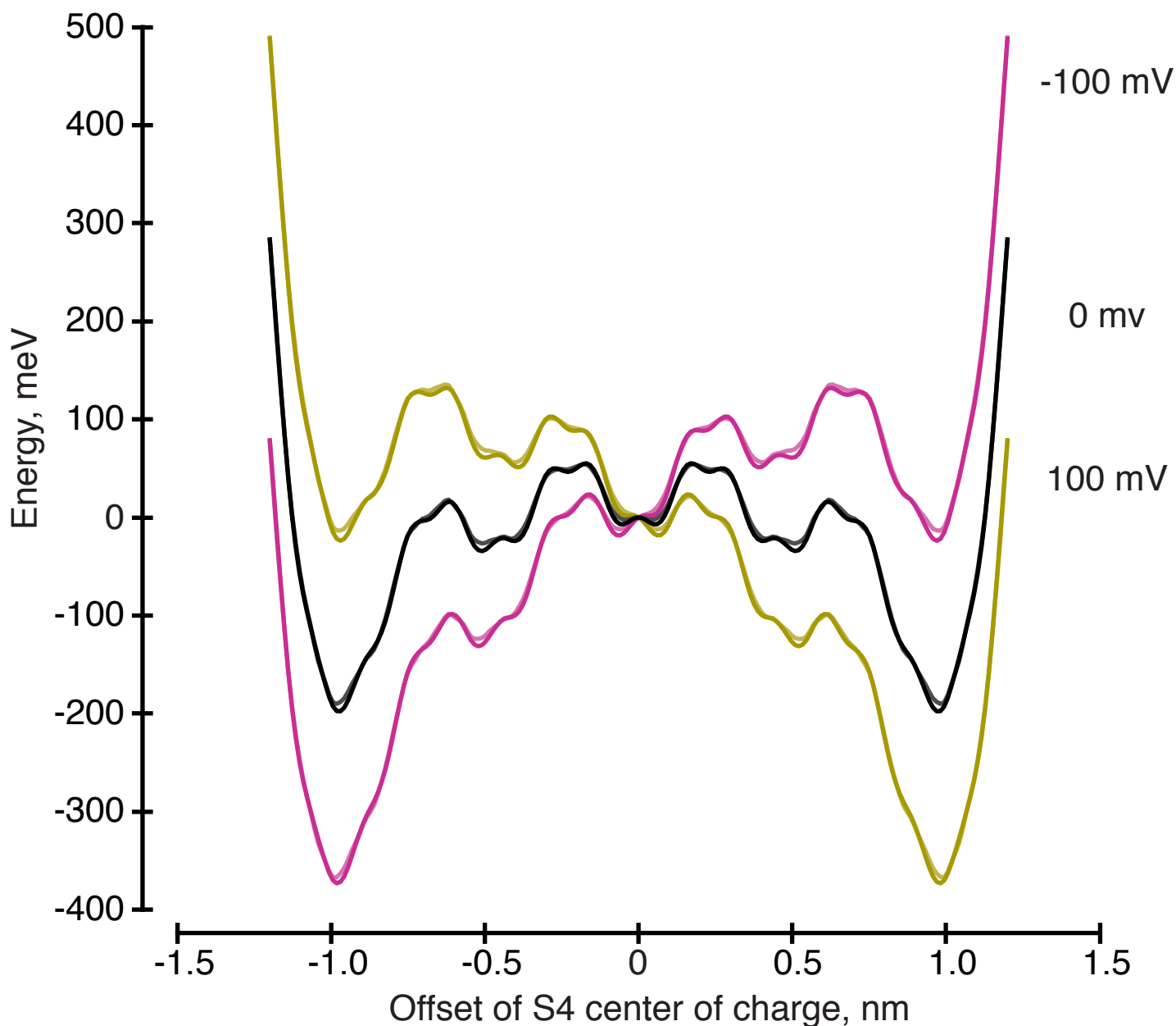
Fig 5 The indicated voltage is applied at the electrodes of the simulation cell. The energy is with respect to that at the center position of the S4 path. The change in energy per applied voltage is the 'effective valency' of an S4 position described in the experimental literature.
