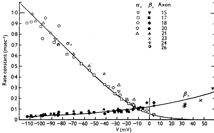
Fig. 4. Abscissa: membrane potential minus resting potential in sea water. Ordinate: rate constants determining rise ( \alpha_n ) or fall ( \beta_n ) of potassium conductance at 6°C. The resting potential was assumed to be 4 mV higher in choline sea water than in ordinary sea water. Temperature differences were allowed for by assuming a Q_{10} of 3. All values for V < 0 were obtained by the method illustrated by Fig. 3 and Table 1; those for V > 0 were obtained from the decline of potassium conductance associated with an increase of membrane potential or from repolarization to the resting potential in choline sea water (e.g. Fig. 2). Axons 17–21 at 6–11°C, the remainder at about 20°C. The smooth curves were drawn from eqns. (12) and (13).
