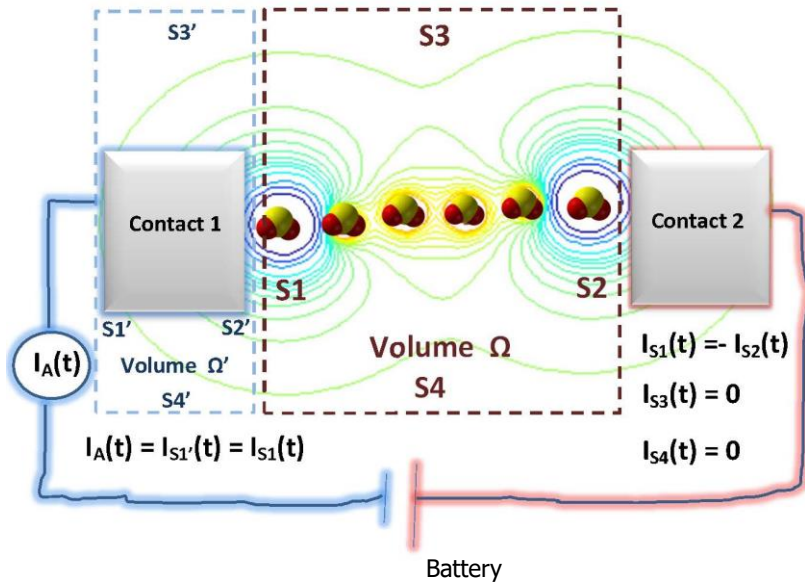
Fig. 1: A two terminal device with a correct selection of the simulation box \Omega that allows a correct computation of the flux of particles and the electric flux on S_1 , I_{S_1}(t) , so that it coincides with the measured current in the ammeter, i.e. I_{S_1}(t) = I_A(t) .
