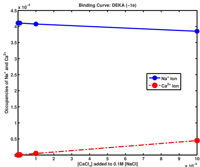
FIG. 3. Binding of sodium to a DEKA channel. This figure shows the relative occupancy of the cylindrical space, that is to say, it shows the ratio of the spatial integral of the density of calcium to the spatial integral of the density of sodium, both within a cylindrical space of 3 Å long and 3.5 Å radius of the stationary solution of the time dependent Euler–Lagrange equations. The concentration of sodium is maintained at 0.1 M on both sides of the channel. The concentration of calcium is varied and is shown on the horizontal axis. The dielectric constant was 80 and the temperature was 298 K. Geometrical setup is nearly the same as Figs. 1 and 2 of Ref. 15.
