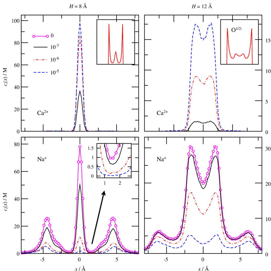
Fig. 5. Axial distribution profiles for \text{Ca}^{2+} (top panels) and \text{Na}^+ (bottom panels) for a short ( H=8 \text{ \AA} , left panels) and a long ( H=12 \text{ \AA} , right panels) selectivity filter at different \text{Ca}^{2+} concentrations ( R=3.5 \text{ \AA} and \epsilon_{\text{pr}}=10 ). The insets of the top panels show the oxygen profiles for [\text{CaCl}_2]=0 \text{ M} . The profiles are symmetric about x=0 because the simulation system is symmetric. Any deviation from symmetry is a result of statistical uncertainty of the simulation. The inset of the bottom-left panel magnifies the depletion zone region as indicated by the arrow. Concentrations are given in M.
