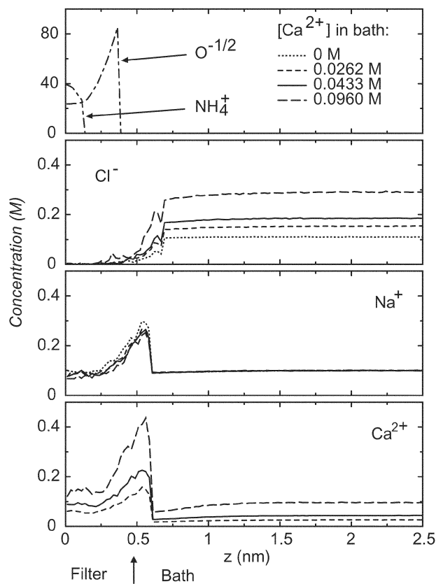
Fig. 5 Axial concentration profiles obtained with the Na channel model in which the NH 4 + ion center is confined to a length of 0.125 nm on either side of the channel center. Profiles are computed as described in Fig. 3.
