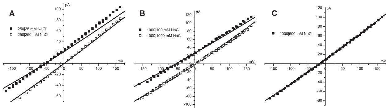
Figure S4. Current/voltage curves in NaCl. Compared to the previous model, the current/voltage curves are more linear and reproduce the data better in very asymmetric solutions. This experimental data was previously published by Chen et al. ( Biophys. J. 76:1346-1366).
