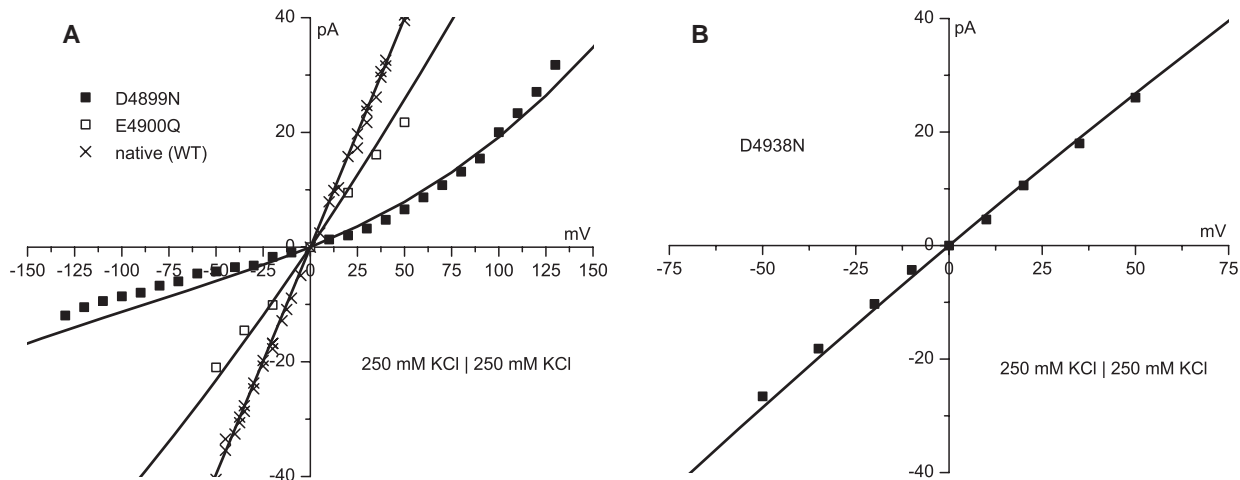
Figure S2. Current/voltage curves of (A) native (WT) RyR (x) and the mutants D4899N (■) and E4900Q (□) and (B) the D4938N mutant in 250 mM symmetric KCl. The D4899N data was previously published by Gao et al. ( Biophys. J. 79:828-840), E4900Q by Wang et al. ( Biophys. J. 89:256-265), and D4938N by Xu et al. ( Biophys. J. 90:443-453).
