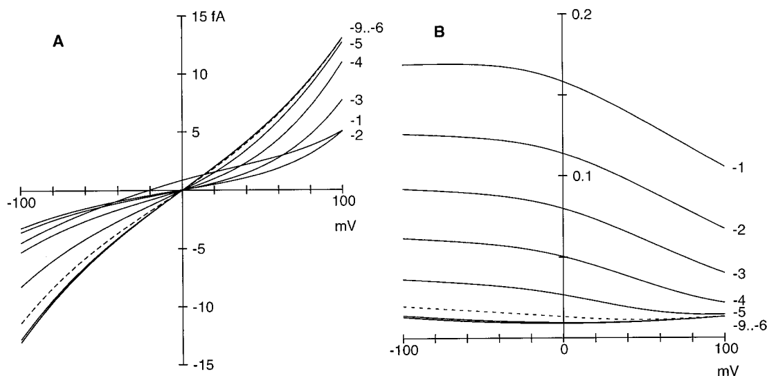
FIGURE 11 Predictions for the step model: current/voltage curves (A) and ionic occupancies (B) at various extracellular Ca concentrations. The solutions contained symmetrical 100 mM NaCl. CaCl_2 was added to only the extracellular solution in 10-fold increments from 10^{-9} to 10^{-1} M (the curves are labeled by the exponent of the power of 10, e.g., -9 for 10^{-9} ; the curves for 10^{-6} M are plotted as dashed lines ). Occupancies give the average number of ions (sum of Na, Ca, and Cl) present in the pore proper.
