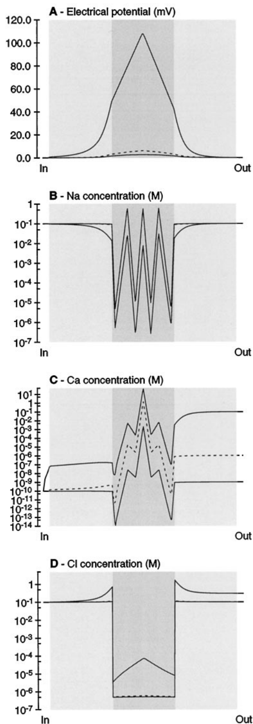
FIGURE 12 Profiles of electric potential and Na, Ca, and Cl ion concentrations as functions of bulk extracellular [CaCl 2 ]. These profiles correspond to the I/V relationships plotted in Fig. 11 A; only the curves corresponding to 10^{-9} , 10^{-6} (dashed lines), and 10^{-1} M Ca are shown for clarity. The transmembrane potential was 0 mV. The abscissa is nonlinear; the bulk section (white background) and atrial sections (light gray) are compressed 100- or 2-fold compared to the pore proper (darker gray). Actual dimensions are given in the body of the paper.
