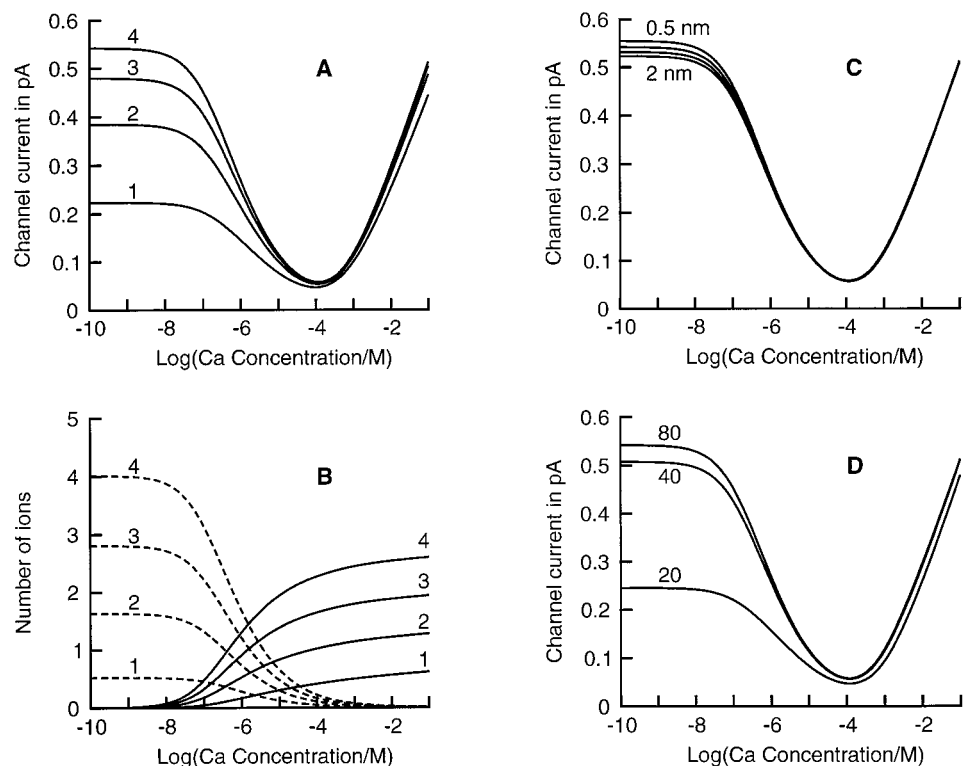
FIGURE 6 Current-AMFE with varied structural parameters. (A) AMFE ( -10 mV) computed for model pores containing one to four carboxyl residues. Other parameters are as given in Table 1. (B) Average number of Na and Ca ions present in the pore proper under the conditions of A. ---, Na ion. —, Ca ion. (C) AMFE computed for various lengths of the pore proper: 0.5, 1, 1.5, and 2 nm. Diffusion coefficients were adjusted in proportion to pore length with respect to the standard values shown in Table 1. (D) AMFE computed for various relative permittivities in the pore proper: 20, 40, and 80. Four carboxyl groups.
