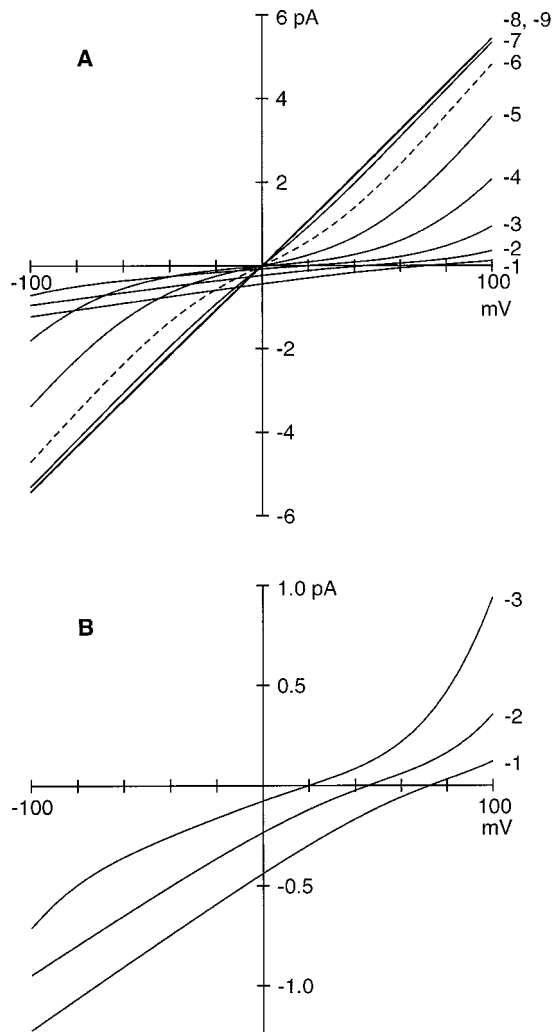
FIGURE 3 Theoretical current/voltage curves at various extracellular Ca concentrations. The solutions contained symmetrical 150 mM NaCl. \text{CaCl}_2 was added to only the extracellular solution in 10-fold increments from 10^{-9} to 10^{-1} M (the curves are labeled with the exponent of the power of 10, e.g., -9 for 10^{-9} ). The pH was 9 on both sides. (A) Plots of the entire set. (B) The three I/V curves computed for 10^{-3} to 10^{-1} M with an expanded current scale. The model parameters are given in Table 1 (four carboxyl groups).
