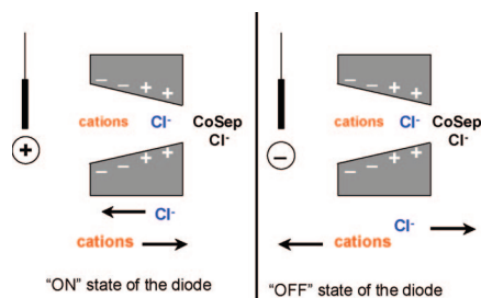
Figure 9. Schematic of an ionic diode with local charge inversion induced by the addition of \text{CoSepCl}_3 at the tip of a conical nanopore. The other opening of the pore is in contact with 10^{-3} M \text{CoSepCl}_3 , so the remaining parts of the pore walls are still negatively charged.
