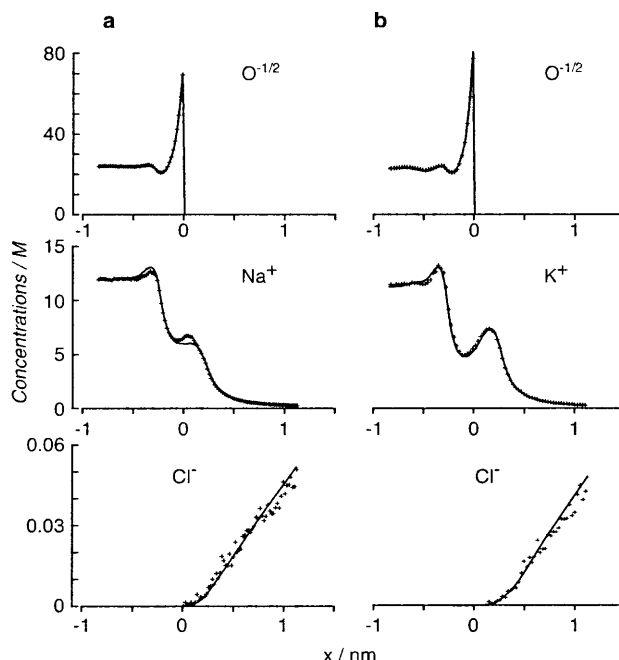
Figure 3. Tests of the DFT for a two-compartment equilibrium problem. (a) The same simulation as in figure 2 except with 0.1 M NaCl in the right compartment with Na + given a diameter of 0.19 nm. (b) The same simulation as in figure 2 except with 22.8 M O 1/2- in the left compartment and 0.1 M KCl in the right compartment with K + given a diameter of 0.266 nm.
