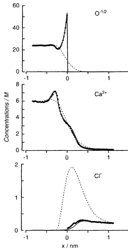
Figure 2. Test of the DFT for a two-compartment equilibrium problem. In the left compartment ( x < 0 ) was a 24 M fluid of half-charged oxygen ions. In the right compartment ( x > 0 ) was 0.1 M of \text{CaCl}_2 . The diameters are \text{Ca}^{2+} 0.198 nm, \text{Cl}^- 0.362 nm and \text{O}^{1/2-} 0.28 nm. The concentrations after equilibration for \text{O}^{1/2-} , \text{Ca}^{2+} and \text{Cl}^- are shown in panels (a), (b) and (c), respectively. In each panel is shown the reference concentration of the ion (dashed curve) used in the final iteration loop (section 4.3). The + symbols represent the results of MC simulations.
