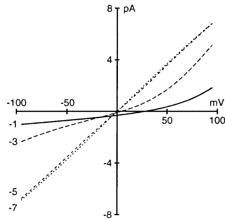
Figure 5. The current/voltage relations for the ionic conditions used in figure 4. The logarithms of the \text{Ca}^{2+} concentration in the right bath are indicated near the curves.
