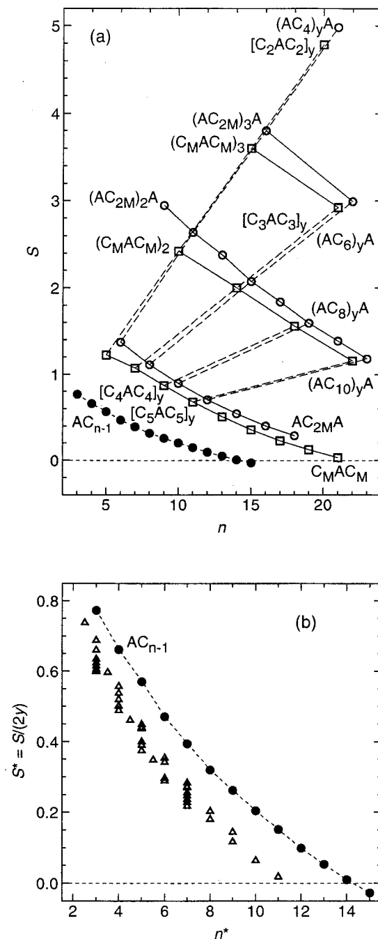
FIGURE 3 (a) Intrinsic potency, S , as a function of solute chain length, n , for alkanols of the general form [C_M AC_M]_y ( \square ) and of the form [AC_{2M}]_y A ( \circ ), where A corresponds to a strongly interfacially active segment ( \epsilon \ll -k_B T , as a model for -CH_2OH or -CHOH- groups) and C to an interfacially inactive segment ( \epsilon = 0 , as a model for -CH_3 or -CH_2- groups). The lines are drawn to group together solutes of a particular type and particular values of either M or y : solid lines for fixed y and varying M , and dashed lines for fixed M and varying y . (b) All results from (a) re-expressed ( \triangle ) as a reduced intrinsic potency S^* = S/(2y) , i.e., the intrinsic potency per amphiphilic subgroup, as a function of the number of segments per subgroup n^* = M + 1 . In both panels, results for solutes of the form AC_{n-1} (models of 1-alkanols) are provided ( \bullet , dotted line). Lipid head group repulsion u_{hg}/k_B T = 0.4 in all cases.
