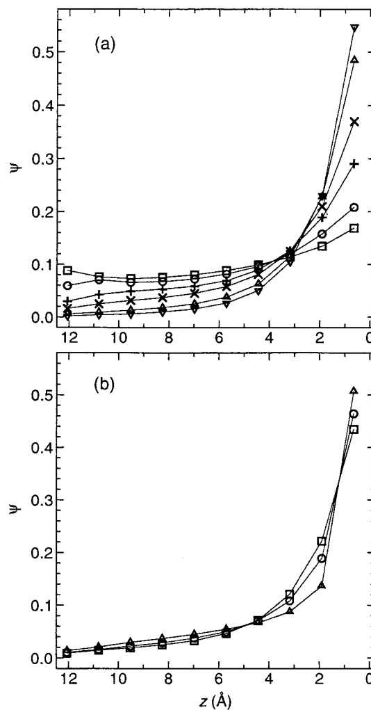
FIGURE 6 Spatial probability distribution \psi(z) of segments of solutes with no interfacial activity ( \epsilon_i = 0, i = 1, \dots, n ) for varying chain length ( n ) and stiffness ( \omega ). Bilayer depth z(\text{\AA}) indicates the distance from the bilayer midplane (in either direction, since the bilayer is symmetric). (a) Semiflexible chains ( \omega = 0.45 ) of length n = 1 ( \square ), 2 ( \circ ), 4 ( + ), 6 ( \times ), 10 ( \triangle ), and 14 ( \nabla ). (b) Fixed alkane chain length n = 8 , for varying chain stiffness: \omega = 0.45 ( \square ), 0.30 ( \circ ), and 0.15 ( \triangle ).
