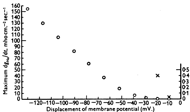
Fig. 11. Maximum rates of rise of sodium conductance during voltage clamps plotted against displacement of membrane potential. Circles are to be read with the scale on the left-hand side. The two lowest points are also re-plotted as crosses on 100 times the vertical scale, and are to be read with the scale on the right-hand side. The peak sodium conductance reached at high strengths of depolarization was 16 m.mho/cm. 2 . Axon no. 41; temperature 3.5° C. Compensated feed-back.
