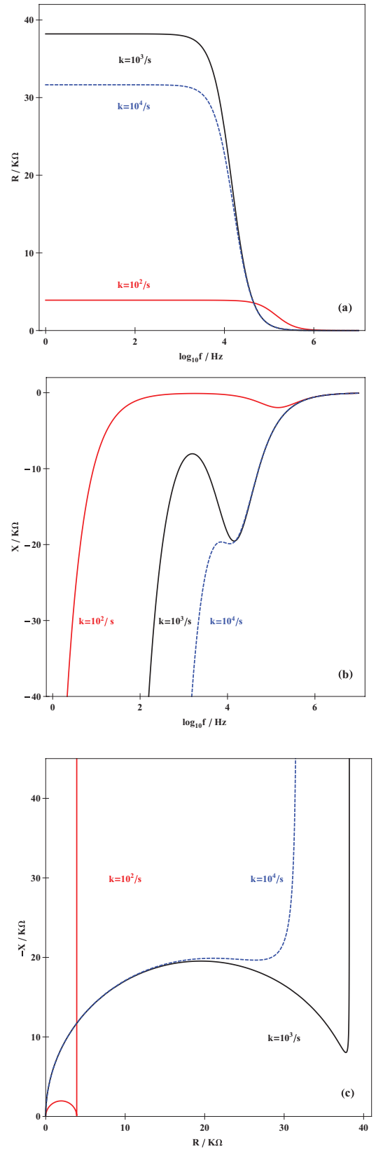
FIG. 7. Frequency dependence of the real, (a), and imaginary, (b), parts of the electrical impedance of the cell for three values of k , and Nyquist plot, (c), when the ions production in the medium is triggered by an external source of energy. For the numerical calculations, we assume that the ions are monovalent, q = 1.6 \times 10^{-19} \text{ A s} , K_B T/q = 25 \text{ mV} , \varepsilon = 80 \times \varepsilon_0 , D = 10^{-10} \text{ m}^2/\text{s} , h = 10^{26} (\text{s m}^3)^{-1} , and k = 10^2/\text{s} , k = 10^3/\text{s} , k = 10^4/\text{s} . The geometrical parameters of the cell are d = 0.5 \times 10^{-3} \text{ m} and S = 10^{-4} \text{ m}^2 .
