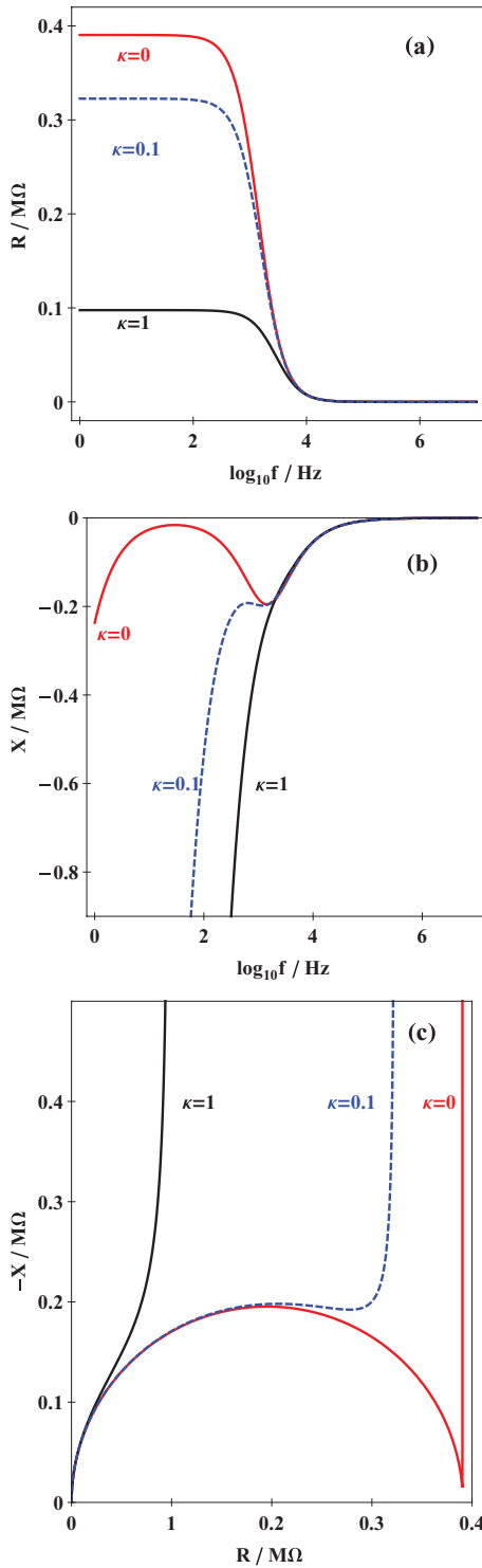
FIG. 1. Spectra of the resistance R = \text{Re}[Z] , (a), reactance X = \text{Im}[Z] , (b), and Nyquist plot, (c), for: full dissociation \kappa = 0 , moderate recombination \kappa = 0.1 , and large recombination \kappa = 1 . For the numerical calculations, we assume that the ions are monovalent, q = 1.6 \times 10^{-19} A s, K_B T/q = 25 mV, \varepsilon = 80 \times \varepsilon_0 , D = 10^{-10} m 2 /s, N_0 = 10^{22} m -3 , and hence \Lambda = 0.105 \mu\text{m} and \omega_D \sim 9 KHz. The geometrical parameters of the cell are d = 0.5 \times 10^{-3} m and S = 10^{-4} m 2 .
