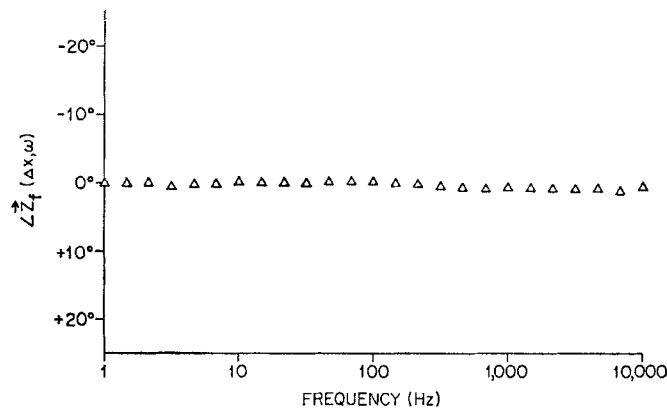
FIGURE 7. Phase angle of the longitudinal impedance, Z_f(\Delta x, \omega) , with respect to frequency. The fiber was chemically skinned. The two gap lengths were 5.0 and 10.0 mm; R_i = 117 ohm-cm. Two other fibers gave similar phase plots and R_i was 124 and 53 ohm-cm.
