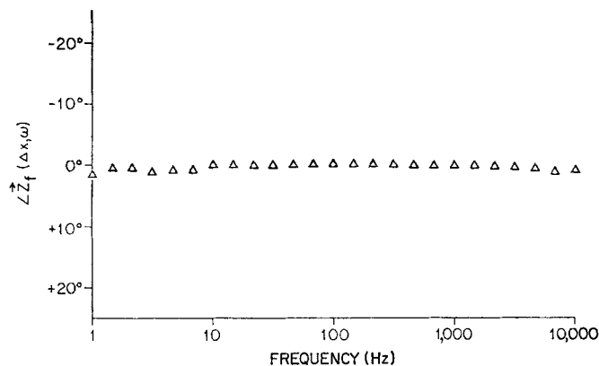
FIGURE 8. Phase angle of the longitudinal impedance, Z_f(\Delta x, \omega) , with respect to frequency. The fiber was mechanically skinned in hypertonic relaxing solution. The two gap lengths were 5.0 and 11.0 mm; R_i = 254 ohm-cm. Another fiber gave a similar phase plot and R_i was 144 ohm-cm.
