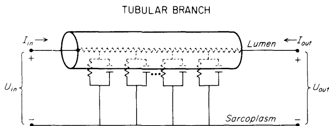
FIGURE 1 The circuit representation of a tubular branch of length L . Each circuit element in the analysis of the mesh model is assumed to be such a distributed network.
