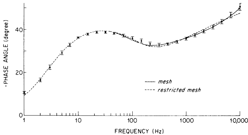
FIGURE 7 The phase angle of the input impedance of frog skeletal muscle fibers. The data is that of Valdiosera et al. (1974c) taken from 12 fibers in their I CCCP solution. Each point is the mean phase measured at that frequency. The standard error of the phase is indicated.
