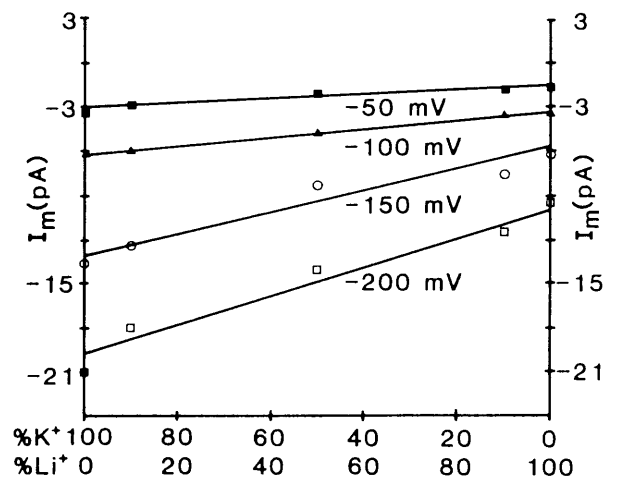
Fig. 10. Li^+/K^+ mole fraction experiment showing no evidence of anomalous behavior. These data were recorded in an on-cell configuration at the indicated patch membrane voltages. The lines are for visual effect only
