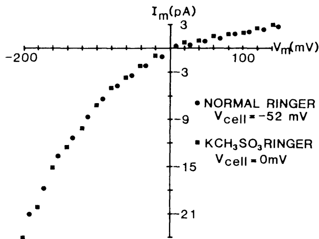
Fig. 7. Open-channel current-voltage relation at different resting voltages. These recordings were made in an on-cell configuration with a 107 mM KCl, minimal \text{Ca}^{2+} , and 10 HEPES solution in the pipette. The cells were depolarized by placing them in a 107 mM \text{KCH}_3\text{SO}_3 (potassium methane-sulfonate) solution
