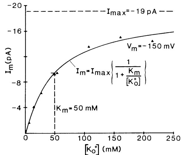
Fig. 9. Current saturation with increasing concentration of permeant ion. These data were recorded in an on-cell configuration with -150 mV across the patch. The solid line represents a fit of the data to a simple Michaelis-Menten saturation function. The best fit was determined by eye. The K_m is 50 mM and I_{max} is -19 pA. The pipette solution contained minimal Ca^{2+} with the indicated [KCl]
