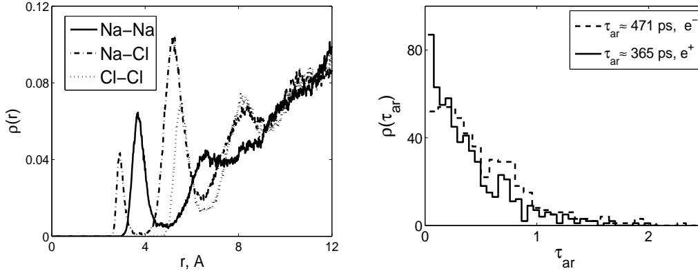
Figure 2. Simulations of Brownian dynamics in the bulk liquid. Left: The number of ions as a function of the distance between ions of different types: C=400 mOsm; Box size: 40 A. Forces included in the simulations were: (i) Coulomb interaction; (ii) short range repulsion; (iii) hydration. Right: The arrival time distribution for positives (solid line) and negative (dashed line) for cylindrical channel of radius r=6 Å
