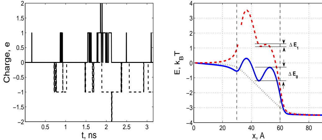
Figure 3. (left) Charge fluctuations at the channel mouth. The positive charge is shown by the solid line. The negative charge is shown by the dashed line. (right) The potential energy profiles as a function of the position of the ion when: the first ion is fixed at the channel mouth (dashed line) and the second is moving along the channel axis. The solid line corresponds to the potential energy on a single ion moving on the channel axis, and the potential energy of the passive channel (dotted line). The vertical dashed lines show the channel entrance and exit. The height of the potential energy barrier seen by a single ion at the selectivity site as it moves from left hand to right hand of the channel is denoted \Delta E_0 . In the presence of a second ion at the channel's left mouth this barrier is reduced to \Delta E_1 .
