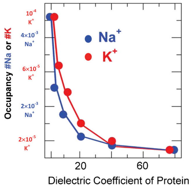
FIGURE 2 Control variables: dielectric coefficient controls contents, i.e., conductance of the DEKA Na channel. Note the different scales on the ordinate for Na + blue and K + red. The solvation energy parameter (the dielectric coefficient ) determines the contents and thus the conductance. The structural parameter (the diameter of the channel ) determines the selectivity (the ratio of Na + to K + ). Each parameter has an effect on one biological characteristic and not on the other. Thus, there are two independent ( orthogonal ) control parameters that control the biological characteristics of the model, independently. Loosely speaking, structure ( diameter ) controls selectivity; solvation ( dielectric ) controls contents and thus conductance. The data shown are unexpected results of 12 simulations, each taking billions of calculations and several days. This figure is redrawn from Fig. 9 of (147).
