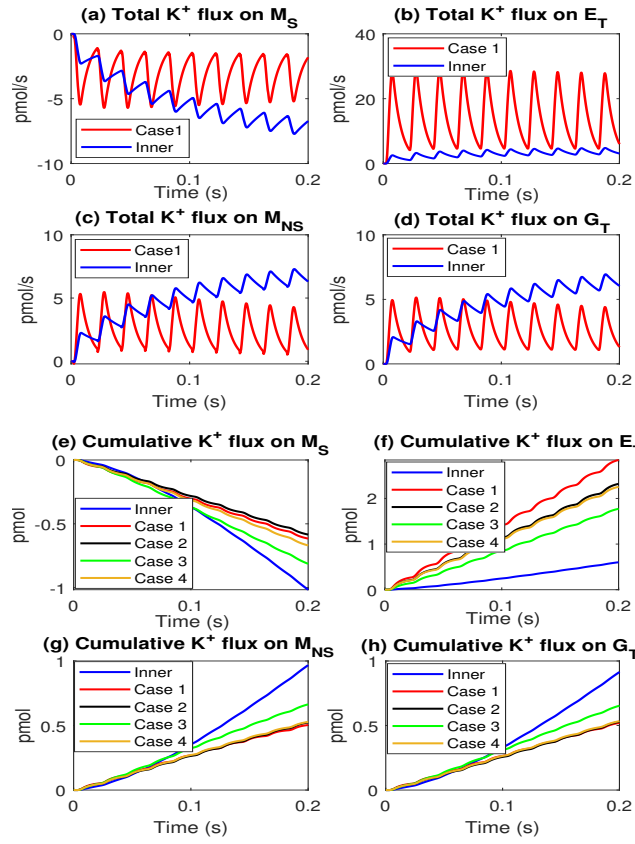
Figure 16: a-d: the comparison between the spatially random stimulated case with the spatially uniform radial (inner) case during a train of axon firing. e-f: the cumulative flux comparison in M_S , E_T , M_{NS} , and G_T during a train of axon action potentials.
