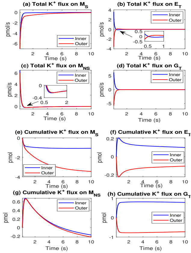
Figure 11: a-d: potassium flux through M_S , E_T , M_{NS} , and G_T after a train action potentials. e-h: cumulative potassium flux after axon firing.
