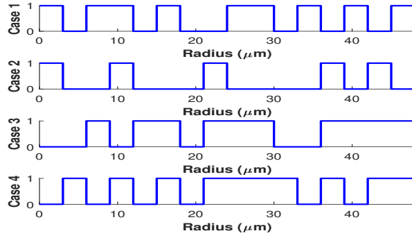
Figure 15: The stimulated radial segments in each case. The intervals with value 1 are stimulated segments and the intervals with value 0 are unstimulated segments.
