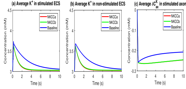
Figure 20: a-b: extracellular potassium concentration variation comparison between the model with NKCC and baseline model (without NKCC). c: average potassium variation in the axon stimulated region.
