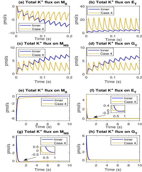
Figure 24: Comparison between spatially randomly stimulated case 4 with the spatially uniform (inner) case.
