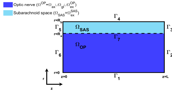
Figure 2: Domain of the axial symmetry model. The optic nerve \Omega_{OP} consist of axon compartment \Omega_{ax} , glial compartment \Omega_{gl} and extracellular space \Omega_{ex}^{OP} . The subarachnoid space only has extracellular space \Omega_{ex}^{SAS} . R_a = 48 \mu m is the radius of optic nerve and R_b = 60 \mu m is the radius from optical nerve center to the dura mater.
