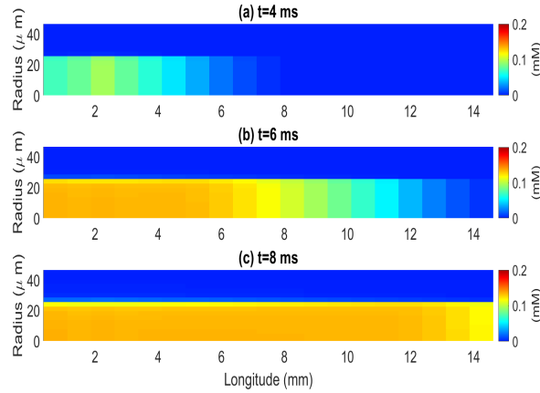
Figure 7: Spatial distribution of potassium changes from the resting state during an action potential.
