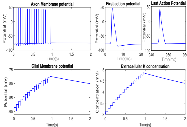
Figure 4: Recording axon membrane potential, glial membrane potential and extracellular K^+ at center axis point (where r = 0 and z = L/2 ) when the extracellular solution with 3 mM K^+ .
