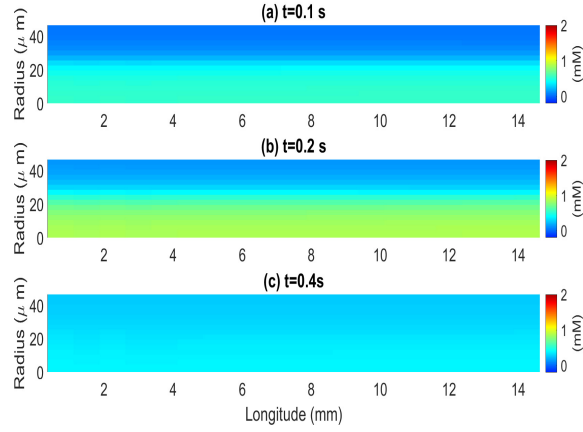
Figure 8: Spatial distribution of potassium changes from the resting state during and after a train of stimuli.
