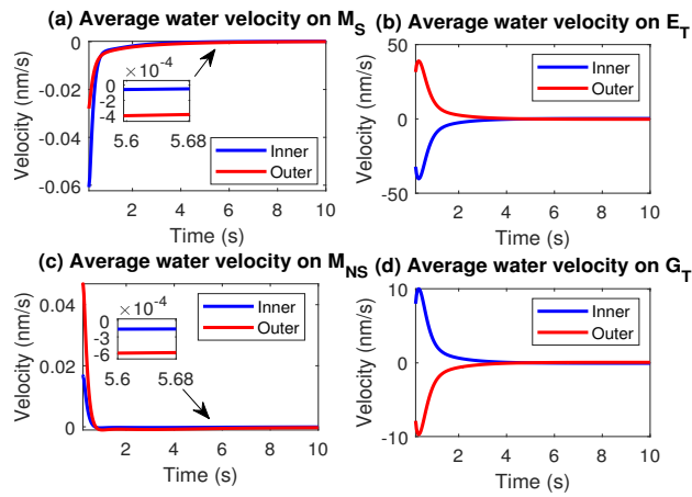
Figure 12: a-d: Average water velocity through M_S , E_T , M_{NS} and G_T after a train of axon firing.
