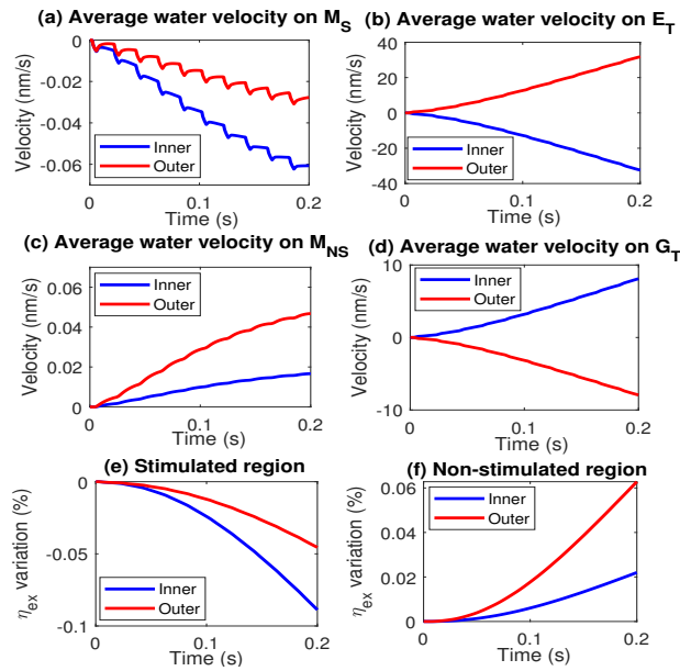
Figure 9: a-d: Average water velocity through M_S , E_T , M_{NS} and G_T during a train of axon firing period [0, T_{sti}] . e-f: the extracellular volume fraction variation in the stimulated region and non-stimulated region.
