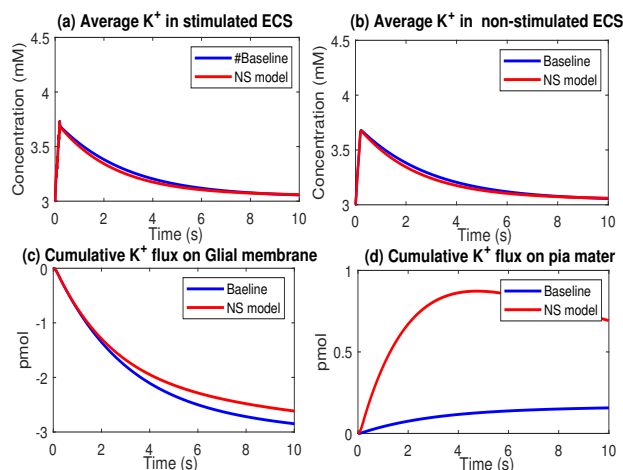
Figure 21: a-b: extracellular potassium concentration variation comparison between the model with non-selective pathway on pia boundary and baseline model (without non-selective pathway).c: total cumulative potassium flux through glial membrane. d: total cumulative potassium flux through pia boundary.
