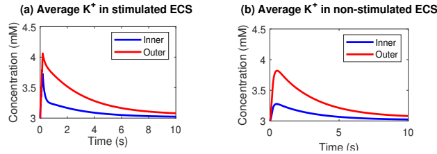
Figure 14: a-b: potassium concentration variation in the extracellular stimulated region and non-stimulated region.
