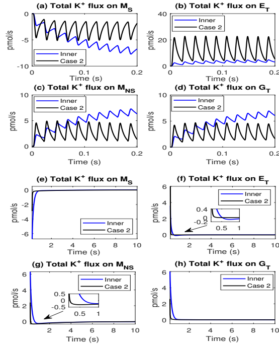
Figure 22: Comparison between spatially randomly stimulated case 2 with the spatially uniform (inner) case.
