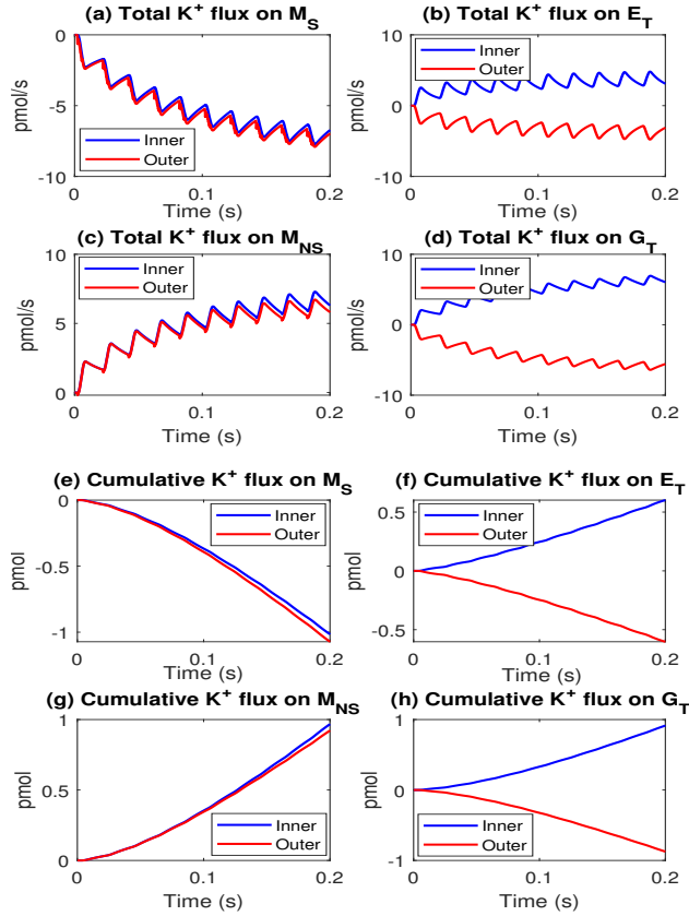
Figure 6: a-d: Potassium flux through M_S , E_T , M_{NS} and G_T during a train of axon firing. e-h: cumulative potassium flux during axon firing period [0, T_{sti}] .
