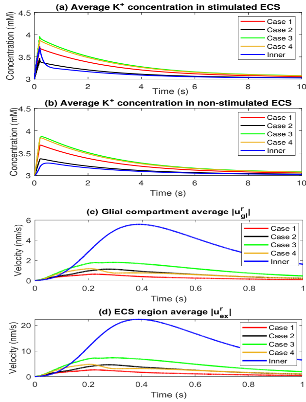
Figure 18: a-b: variation of potassium concentration in the extracellular simulated region and unstimulated regions. c-d: average glial compartment radial absolute velocity and extracellular space radial absolute velocity.
