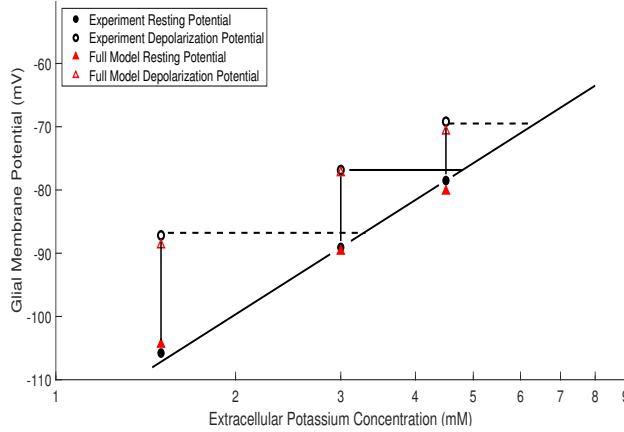
Figure 5: Comparison between the experiment in [53] and simulation on the effect of nerve impulses on the membrane potential of glial cells. The solid symbols are resting potentials and the open symbols are depolarization potentials with different K^+ concentrations in \Omega_{ex}^{OP} .
