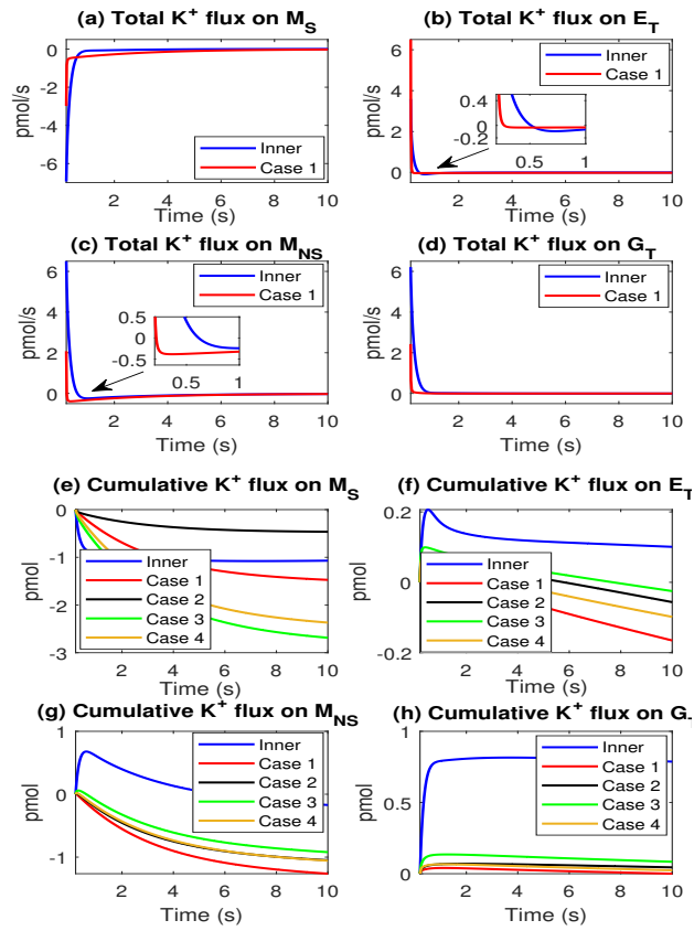
Figure 17: a-d: the comparison between the spatially random case with the uniform inner radial case after a train of action potentials Vector directions as defined previously. e-f: the cumulative flux comparison in M_S , E_T , M_{NS} , and G_T after a train of action potentials.
