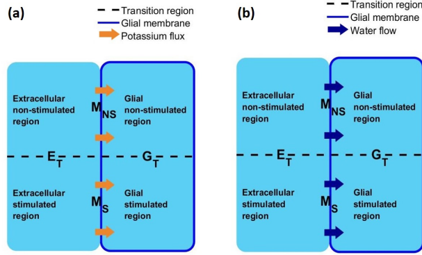
Figure 13: a: Schematic graph of the potassium flux after the axon was stimulated. The potassium flux leaks into the glial compartment from the extracellular space through the glial membrane in both stimulated and unstimulated regions. The potassium flux in the extracellular space and glial compartment is negligible. b: Schematic graph of the water flux after the axon was stimulated. Note these graphs are graphs that summarize outputs of large numbers of calculations solving partial differential equations in longitudinal and radial spatial directions and time. They do not represent a compartmental model. They are the output of a model distributed in space.
