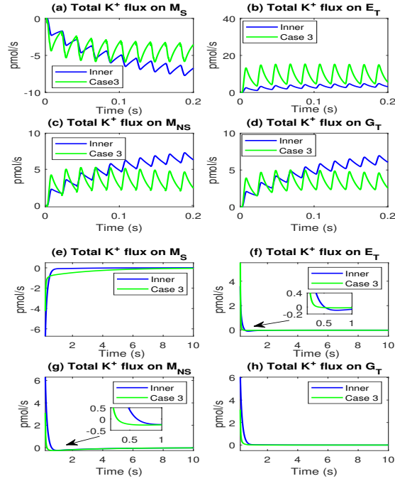
Figure 23: Comparison between spatially randomly stimulated case 3 with the spatially uniform (inner) case.
