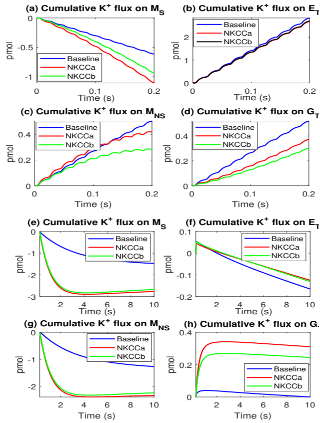
Figure 19: a-d: the cumulative flux comparison in M_S , E_T , M_{NS} , and G_T during a train of action potentials. e-h: the cumulative flux comparison in M_S , E_T , M_{NS} , and G_T after a train of action potentials.
