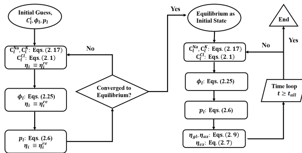
Figure 3: Flowchart for simulation process
