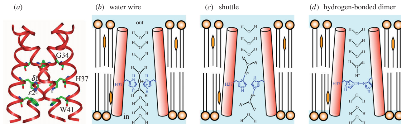
Figure 6. The well-studied M2 proton channel of influenza A virus is a homotetramer; (a) shows the high-resolution crystal structure with key residues labelled. Three proposals for the proton selective conduction are illustrated in (b–d), with only two of the four protomers shown for clarity. In the water wire model (b), the proton pathway is exclusively aqueous, with protonation of multiple His 37 serving to open the pore by electrostatic repulsion. Proton selectivity in the shuttle model (c) is achieved by successive protonation and deprotonation of His 37 , with a ring flip completing each conduction event. In (d) protonated and unprotonated His 37 form hydrogen-bonded dimers that are broken during H + conduction. (Adapted from [139].)
