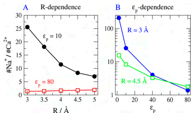
FIGURE 10 The ratio of the occupancies of Na + and Ca 2+ ions (A) as a function of pore radius R for two different protein dielectric coefficients of the protein ( \epsilon_p = 10 and 80) and (B) as a function of \epsilon_p for two different radii of the pore ( R = 3 and 4.5 Å). The bath Ca 2+ concentration is 17.5 mM. Protein dielectric coefficient has little effect on Na + versus Ca 2+ selectivity when the protein dielectric coefficient is large, but it has a substantial effect when the protein dielectric coefficient is small. The radius of Na + and Ca 2+ are nearly the same ( r_{\text{Na}^+} = 1 , r_{\text{Ca}^{2+}} = 0.99 Å) so this graph shows charge selectivity. The selectivity filter has spatially nonuniform selectivity (see Fig. 7) and so we define and plot occupancy in the central most-selective region of the filter \pm 2.5 Å from the center of the pore.
