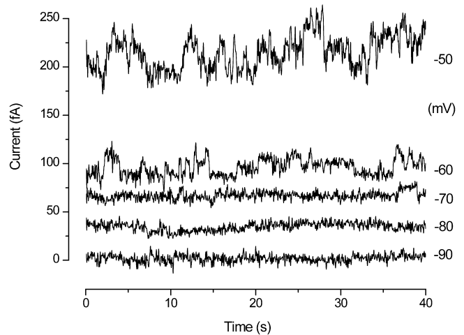
FIGURE 9. Apparent single proton channel currents at pH_o 7.5 and pH_i 5.5. These currents were filtered at 20 Hz (8-pole Bessel) and later digitally refiltered at 10 Hz. The current scale is positioned arbitrarily. The resistance of this patch at subthreshold voltages was 5 T \Omega . For clarity, each record is displaced vertically by 20 fA above its true position relative to the record underneath. ES2724.
