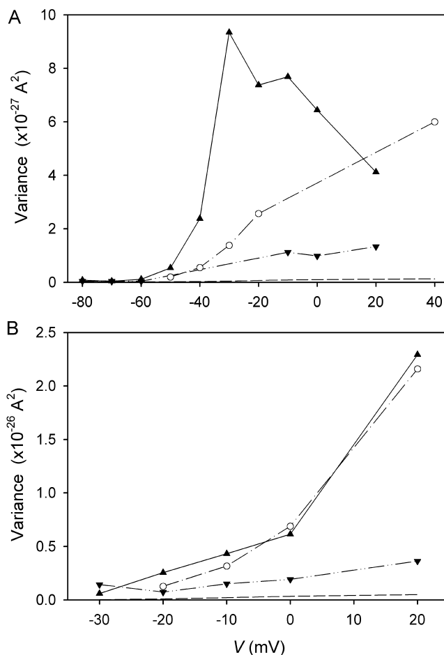
FIGURE 11. The Lorentzian variance ( \blacktriangle ) and the band-limited 1/f variance ( \circ ) and white noise ( \blacktriangledown ) variances were determined from fitted power spectra (Fig. 10) and are plotted here against membrane voltage ( V ). The white noise and 1/f variances were calculated over the interval [f_0, f_N] , where f_0 is the lowest frequency in the spectrum and f_N is the Nyquist frequency. On average, the band-limited Lorentzian variance (open symbols in Fig. 4) was \sim 10\% less than the total Lorentzian variance (which is plotted here). The dashed lines without symbols show the calculated sum of the Johnson- and shot-noise variances (see Fig. 10) over the interval [f_0, f_N] . (A) pH_o = 7.5 , pH_i = 5.5 , V_{\text{threshold}} = -55 mV; (B) pH_o = 7.5 , pH_i = 6.5 , V_{\text{threshold}} < -30 mV. Same two patches as in Fig. 10. In A, 1/f noise was not detectable between -10 and 20 mV; presumably it was masked by the Lorentzian. On the other hand, only 1/f noise was detected at 40 mV; apparently Lorentzian noise had fallen to undetectable levels, suggesting a P_{\text{max}} value close to unity. In B, no peak is observed in the Lorentzian variance, suggesting P_{\text{max}} \leq 0.8 (see text and Fig. 5).
