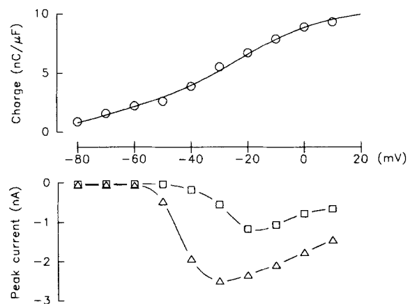
FIGURE 5. Voltage dependence of charge movement and ionic currents. Circles , ON charge (time integrals of ON transients in Fig. 4 C); triangles , peak amplitudes of \text{Na}^+ current; squares , peak \text{Ba}^{2+} current. Data for ON charge fitted by the equation:
