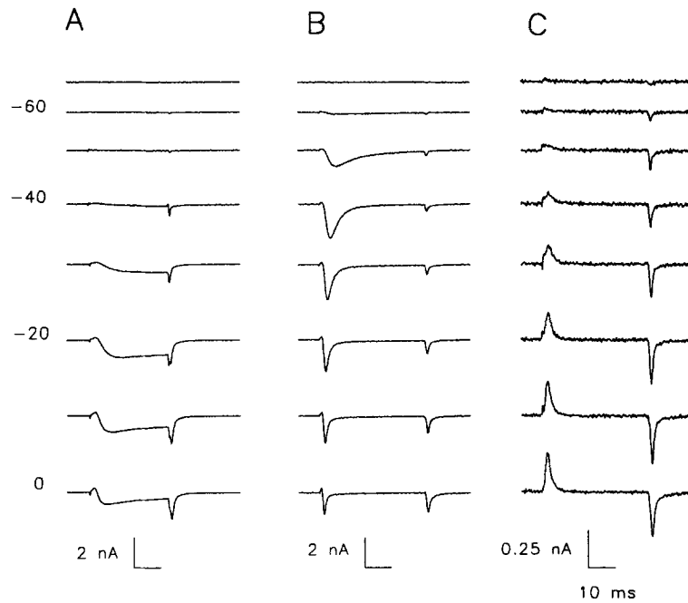
FIGURE 4. Charge movement and activation of \text{Ba}^{2+} and \text{Na}^+ currents. Currents elicited by pulses from h.p. -110 mV to the voltages indicated. (A) \text{Ba}^{2+} currents; records obtained after 3.5 min of cell perfusion with Barium solution. (B) \text{Na}^+ currents; recorded in Sodium solution after rundown of \text{Ba}^{2+} currents. (C) Asymmetric currents in the same cell perfused with Charge movement external solution. Note change of scale in C. Cell #91822C15; C_M = 132 pF.
