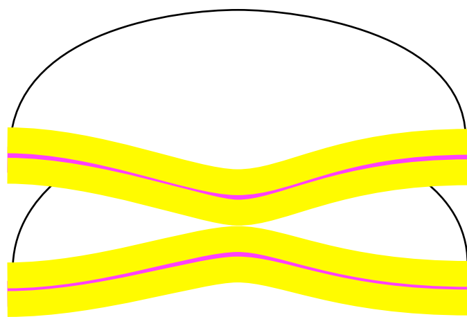
nipples
