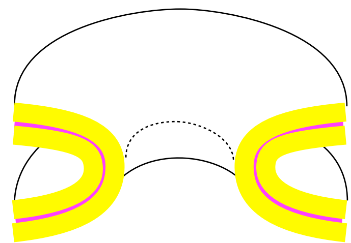
enlarged pore
