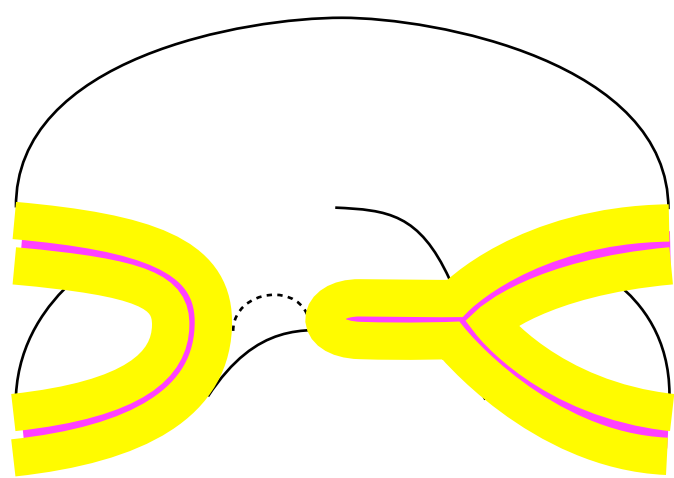
initial pore
