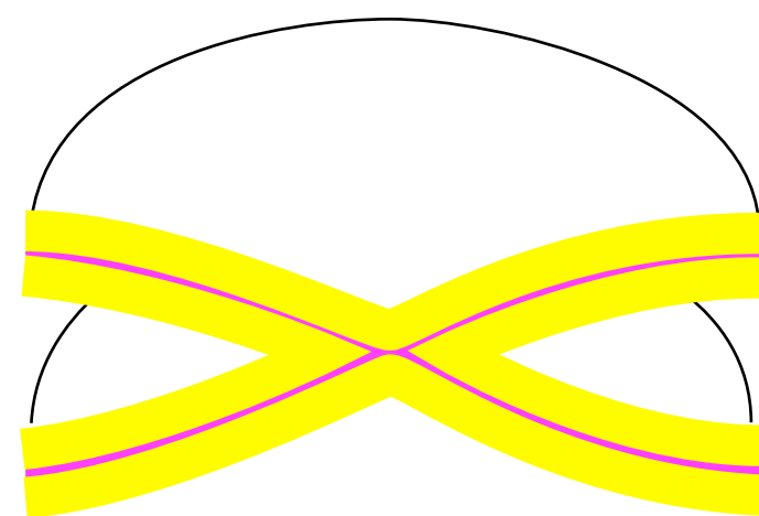
stalk
